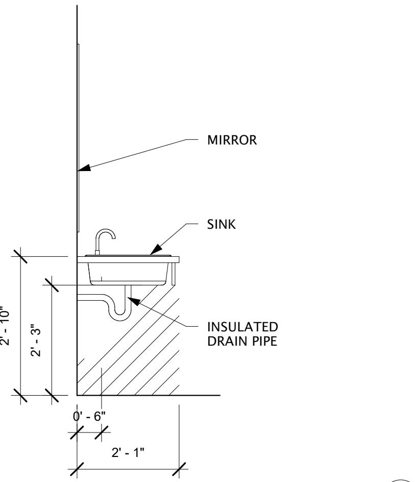
SINK ELEVATION - SIDE 1/2" = 1'-0" (3C)
