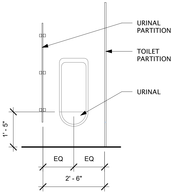
URINAL ELEVATION - FRONT 1/2" = 1'-0" (5A)
