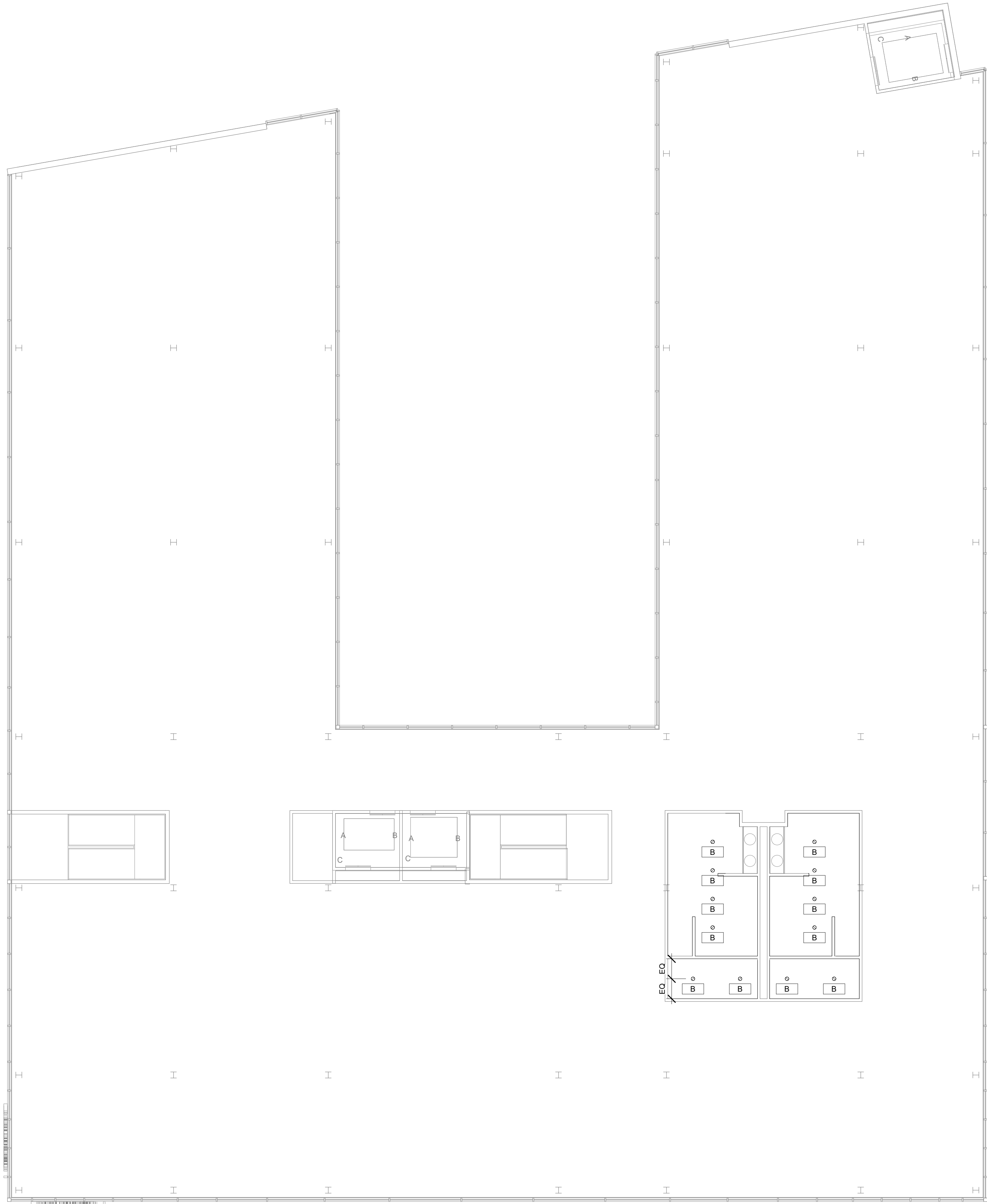
SECOND FLOOR CEILING PLAN 1/8" = 1'-0"
