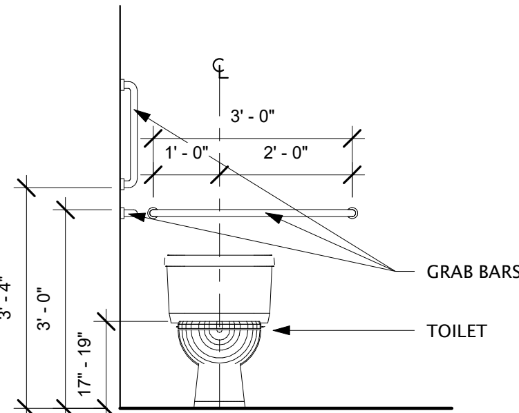
TOILET ELEVATION - FRONT 1/2" = 1'-0" (1A)
