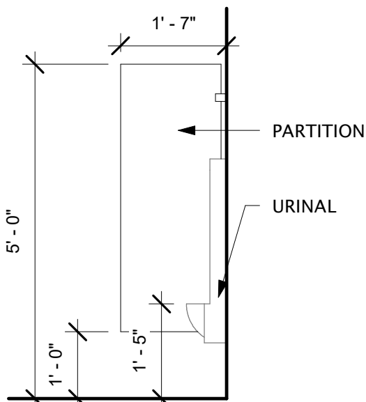
URINAL ELEVATION - SIDE 1/2" = 1'-0" (7A)
