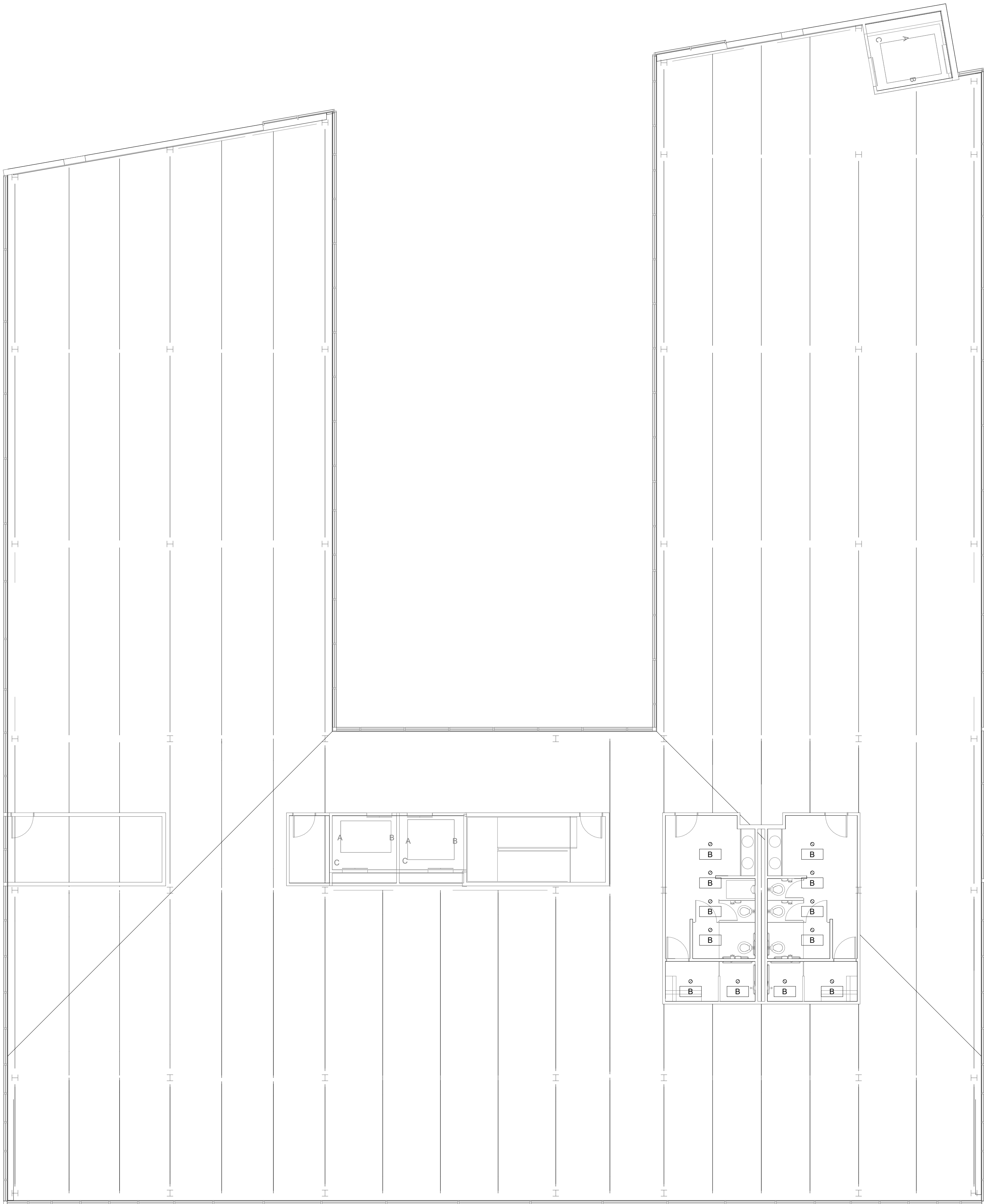
THIRD FLOOR CEILING PLAN 1/8" = 1'-0"
