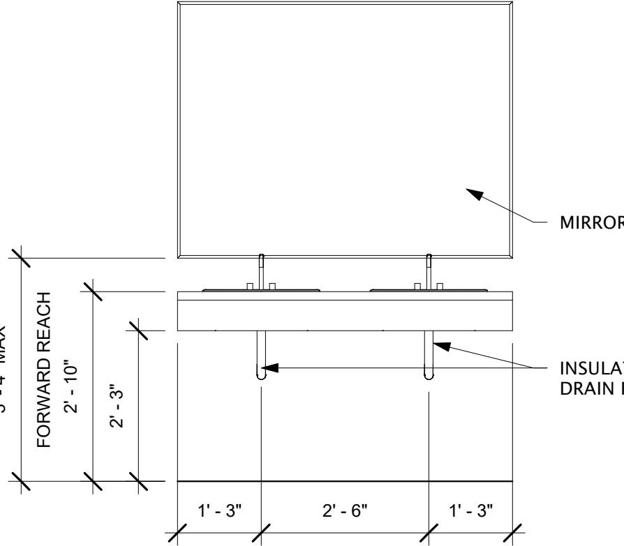
SINK (DOUBLE) ELEVATION - FRONT 1/2" = 1'-0" (1C)
