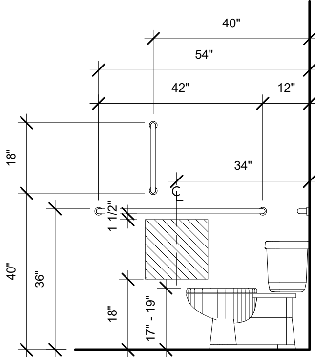
TOILET ELEVATION - SIDE 1/2" = 1'-0" (2A)
